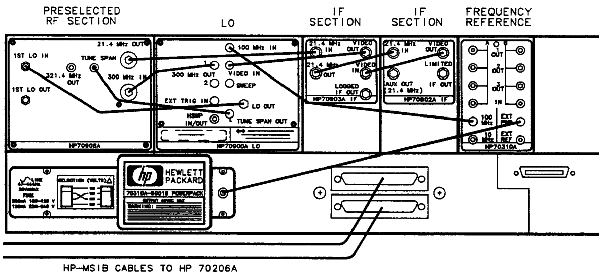
Figure 2-4. HP 71210A Microwave Spectrum Analyzer Rear-Panel Cables
